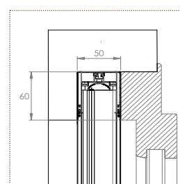
■ BORA TOP INCAS STANDARD 50/50
