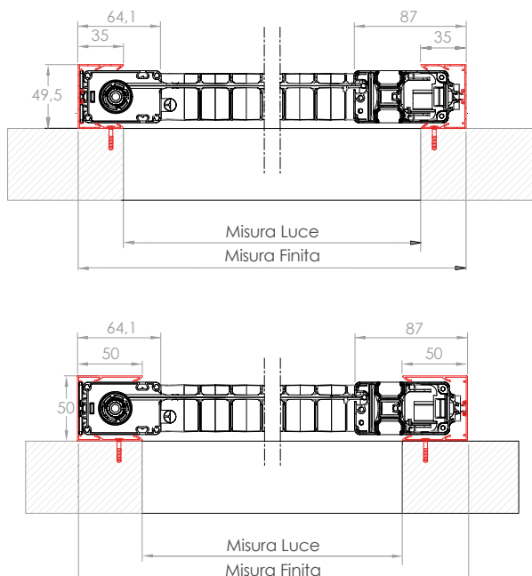
■ BORA TOP UP STANDARD 35/35 - 50/50
