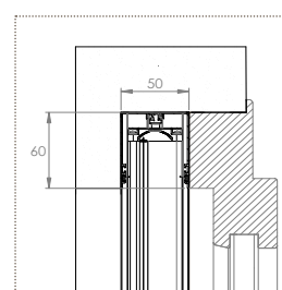
■ BORA TOP INCAS STANDARD 50/35
