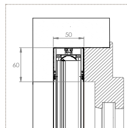
■ BORA TOP INCAS STANDARD 50/20
